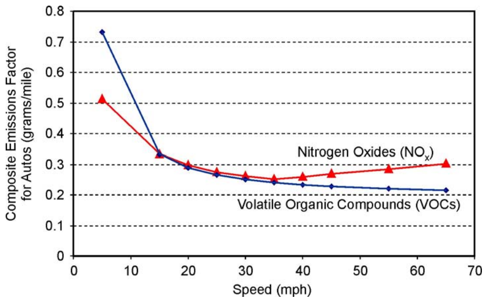
Figure 2. Composite Emissions Factors for Automobiles.
