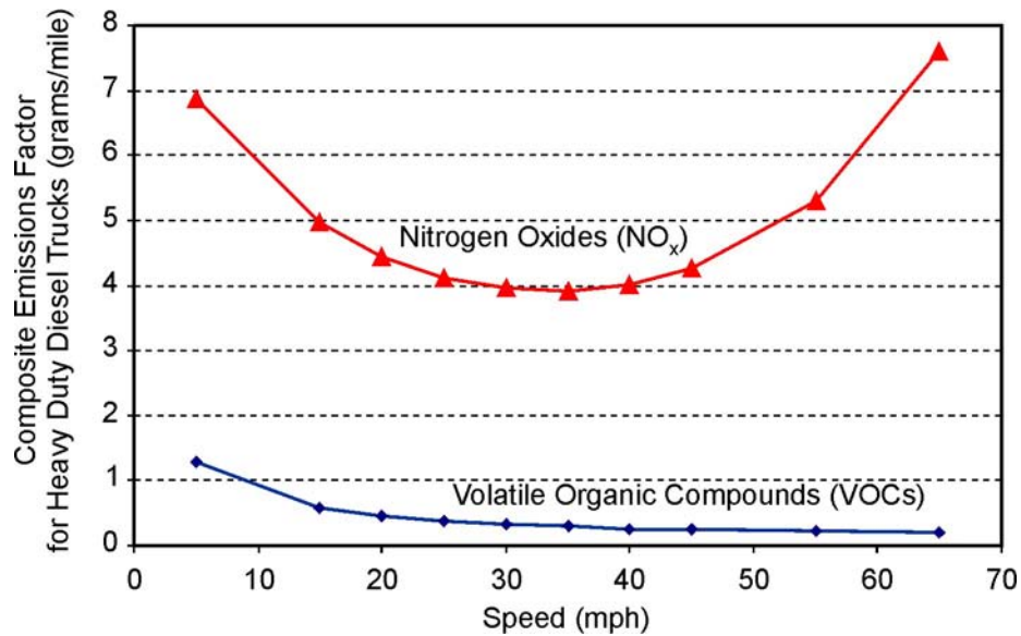
Figure 3. Composite Emissions Factors for Heavy Duty Diesel Trucks.
